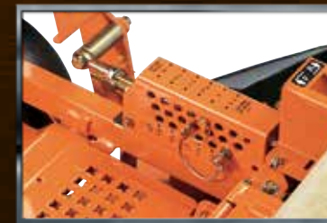
Foot pedal deck lift makes changing the height-of-cut fast and easy. Adjusts from 1" to 5" in 1/4" increments.
