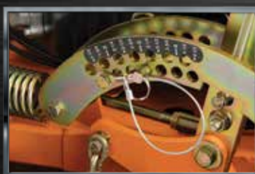
Easily change cutting heights in the field with no tools (1 1/2" to 4 1/2" in 1/4" increments). Deck can be lifted from the operating position with the pull of a spring-assisted lever.
