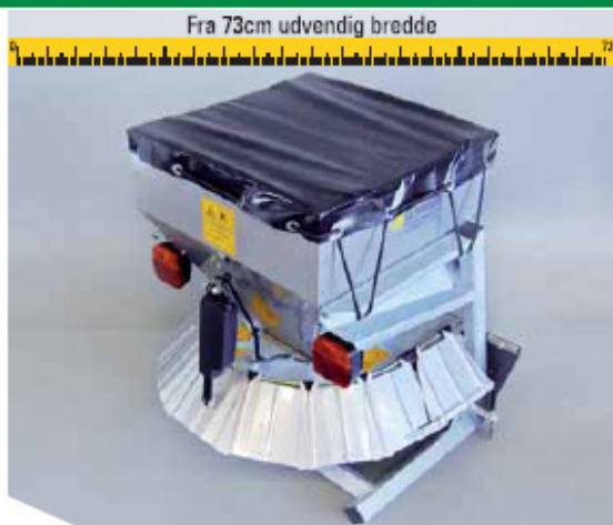
Tallerkenspreder ECO-XTA-140
